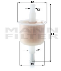
Fuel Filter WK 32 EM-20037
