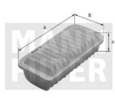
Air Filters C 25 017 EM-30250
