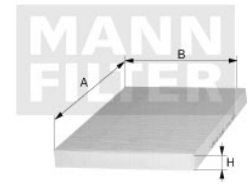
Cabin Air Filter FP-M09 EM-40166
