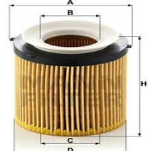
Oil Filter HU 8002 x KIT EM-10100
